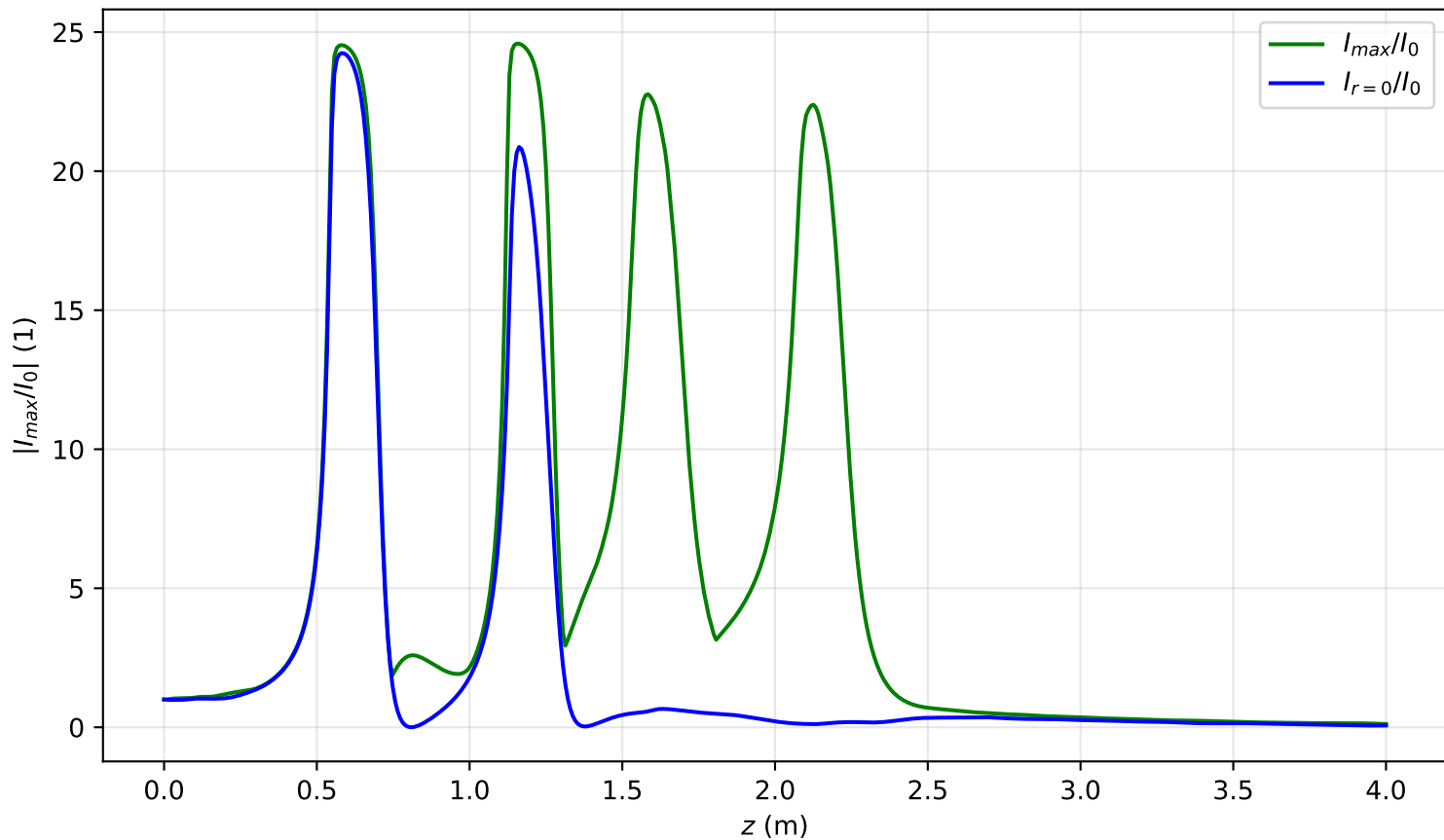
I_{max}(x=0, y=0, z)/I_0 , P_{in}=4.5P_{cr} , noisy input, artificial time
